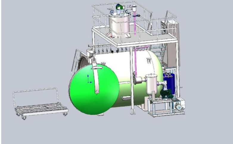
2. KCY-400-II vacuum pressure casting (the most commonly used in China)
