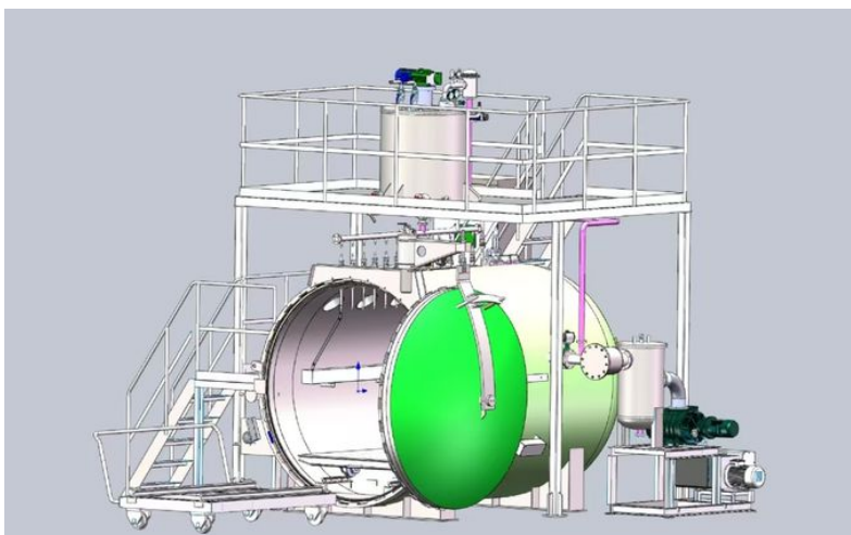
3. KCY-400-I vacuum pressure casting (four columns on the tank body for easy installation)
