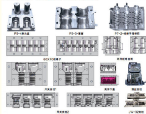
环氧树脂压模模具 Epoxy Resin Clamping Molds
